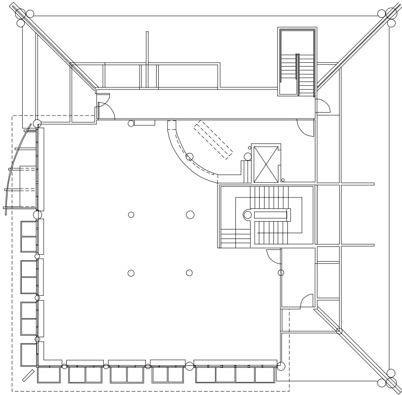
2nd Floor
